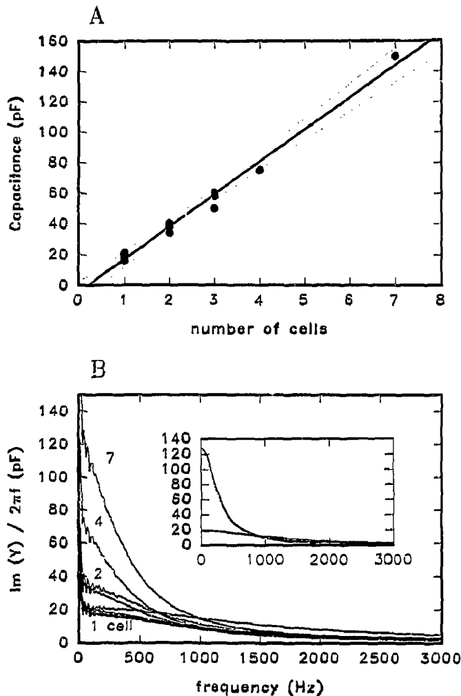
Fig. 3. A. Relationship between whole-cell capacitance, measured 15 min after lowering pH, and number of cells in the cell aggregate which included the patch-clamped cell. Linear regression (shown as a solid line with 95% confidence bands) yields an average value of 21 pF for single cell capacitance, which compares well to that measured for single cells ( 19 \pm 0.9 ). We used the cell medium as external solution and a KCl buffer as internal solution (150 mM KCl, 7 mM MgCl 2 , 10 mM HEPES, 1 mM EGTA, pH 7.2). B. The imaginary part of whole-cell admittance, normalized with respect to the angular velocity, is given for a number of cells in mutual contact. The whole-cell recording technique was used on one cell [9]. Zero frequency intercepts estimate different capacitance values before and after lowering pH. Pseudo-random binary voltage signals (0–10 mV), having a quasi-white spectral density (5 kHz bandwidth), were used to determine the complex admittance of the cell membrane [13]. The measured admittance was consistent with the simple equivalent circuit of a series resistance of the pipette and a parallel capacitor/resistor of a single syncytial membrane (inset, showing prediction of this circuit).
